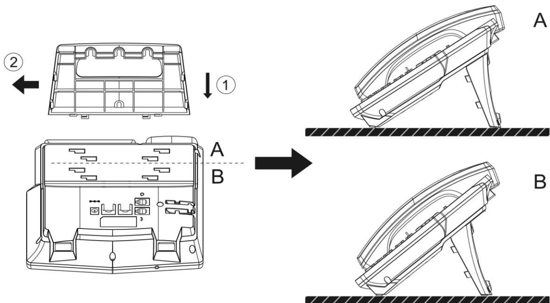
Figure 1 - Desktop Installation
